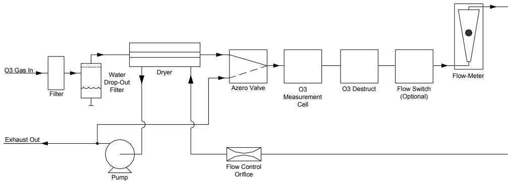
Figure 2-1: Pneumatic Diagram (Rack Mount Version)
