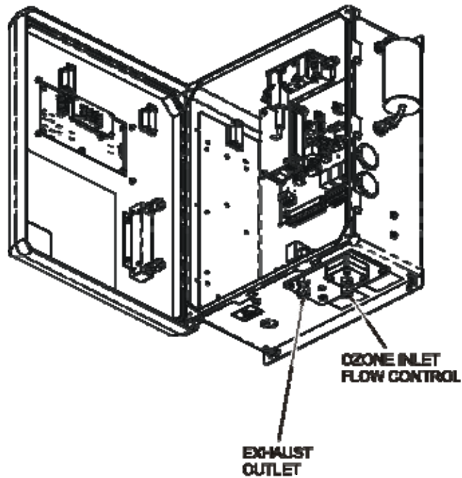
Figure 2-4: Pneumatic Connections, NEMA Configuration
