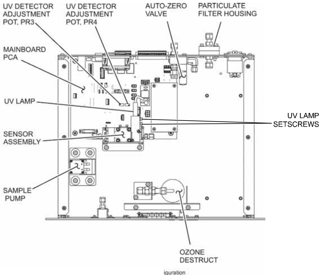
Figure 3-1: Instrument Layout, Rack Mount Configuration
