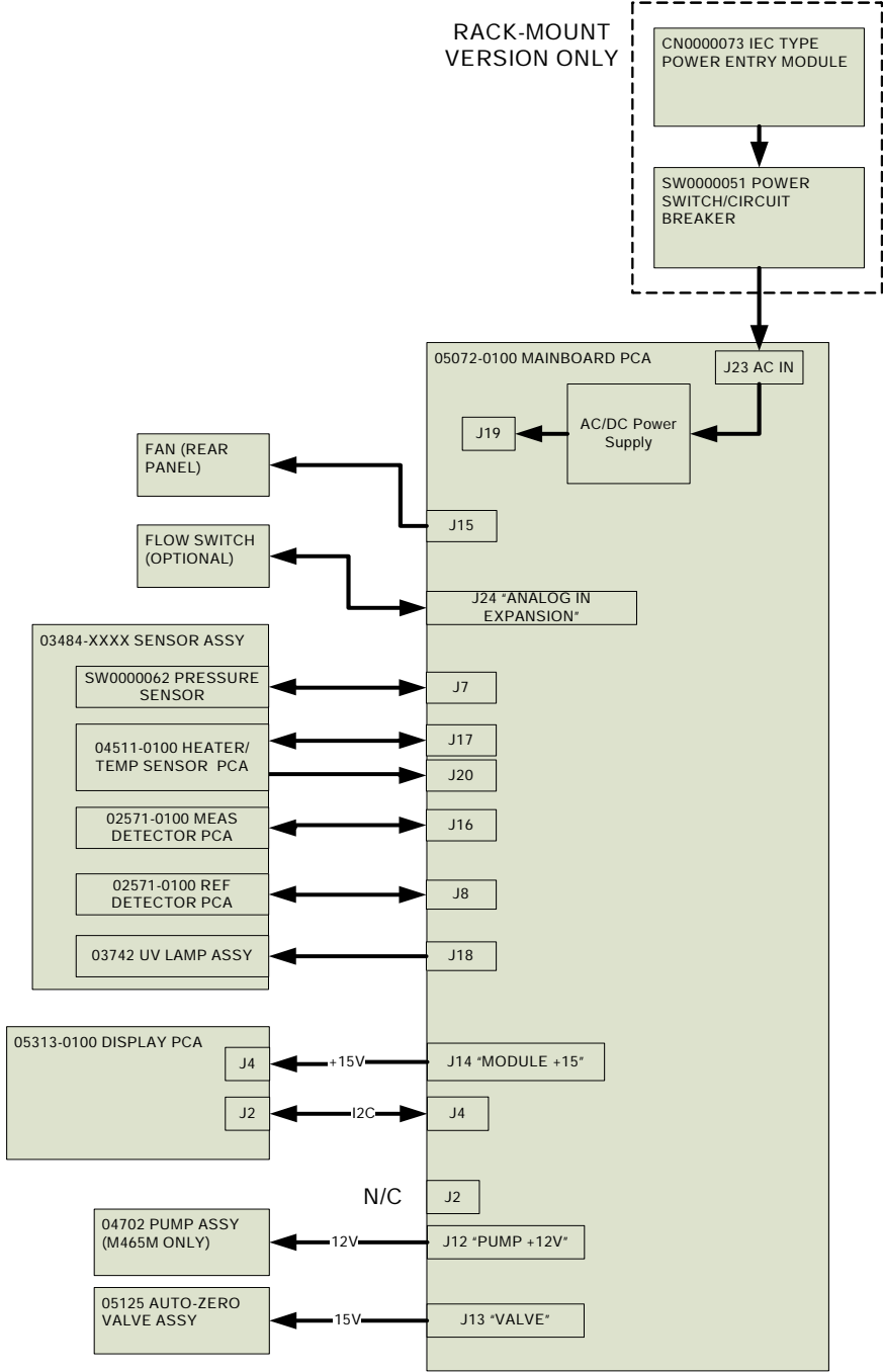
Figure 7-3: Interconnect Diagram
