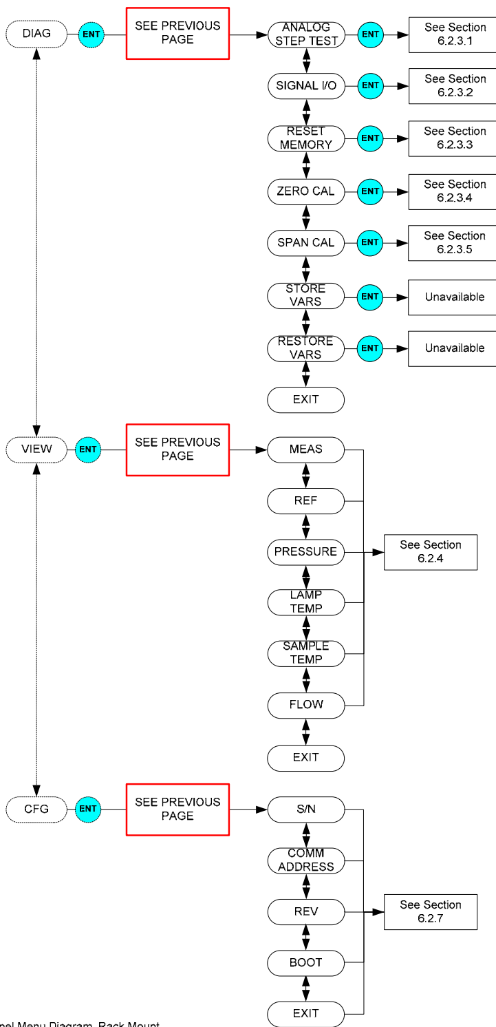
M465M-Front Panel Menu Diagram, Rack Mount
