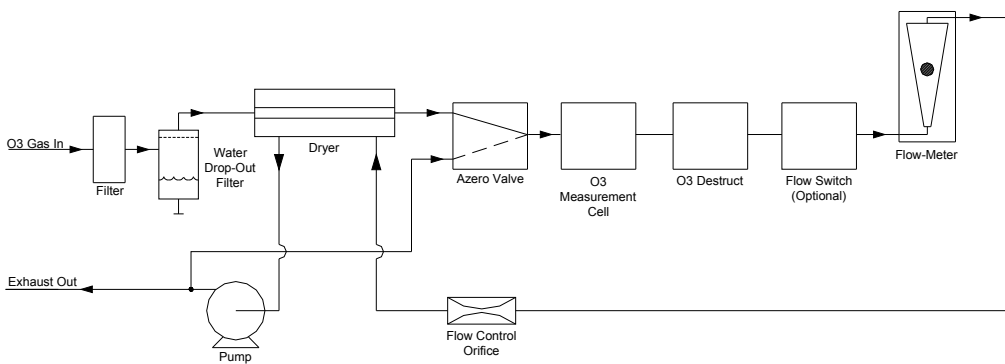
Figure 7-2: Pneumatic Diagram (NEMA Version with Sample Conditioner)
