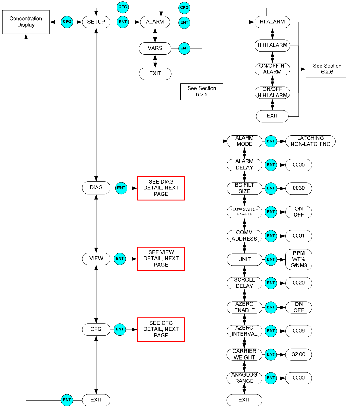
M465M-Front Panel Menu Diagram, Rack Mount
