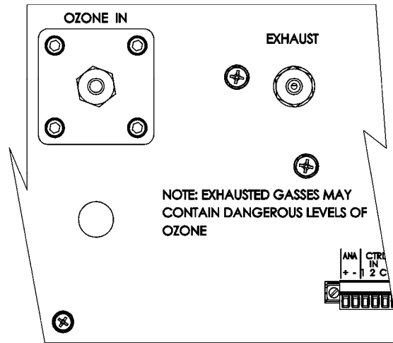
Figure 2-3: Pneumatic Connections, Rack Mount Configuration
