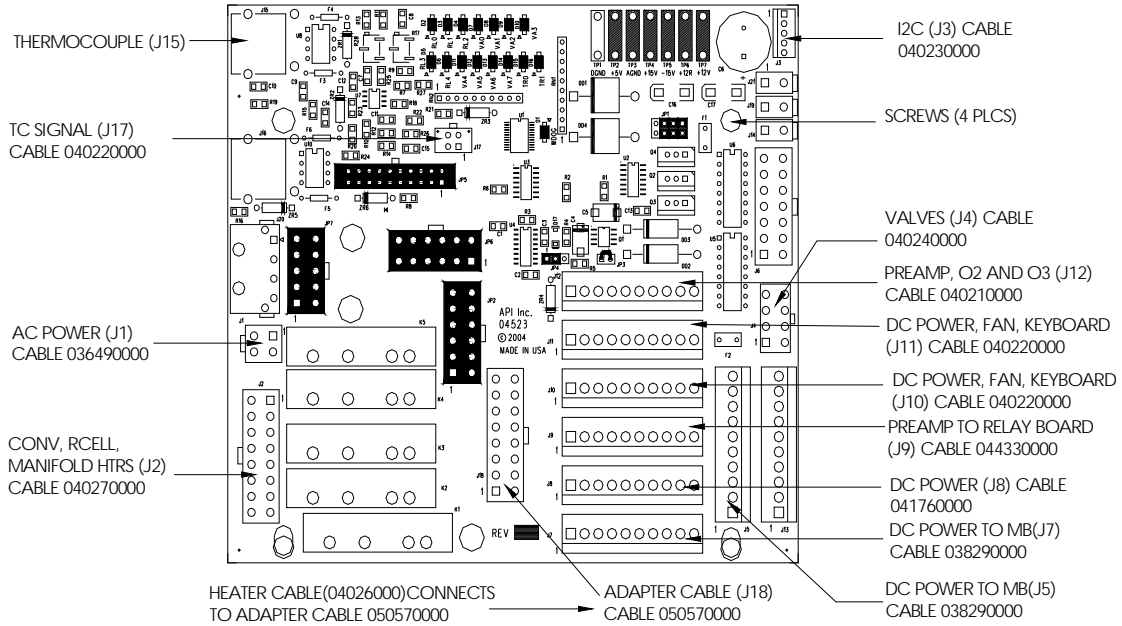
FIGURE 4 CONNECTING THE ADAPTER CABLE
