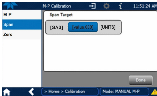
Figure 3-9. Calibration Span Target Page (with valve option)
